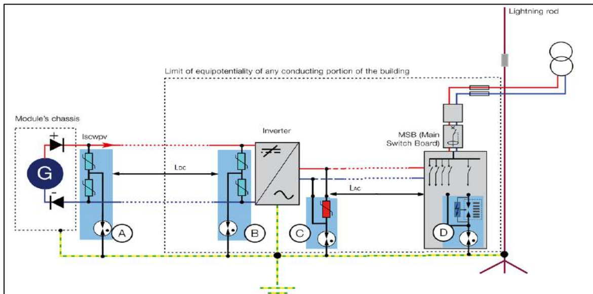
Figure 3 5: Recommended SPD locations of PV installation
